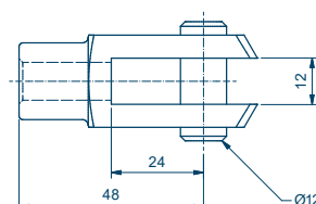
Fork Joint
