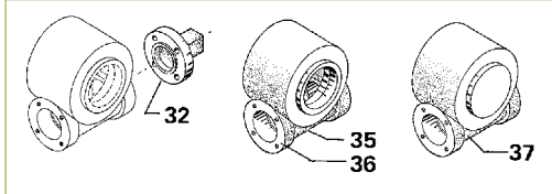
Housing type 1
