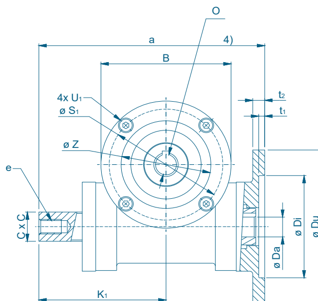
Hollow shaft and mounting threads left
