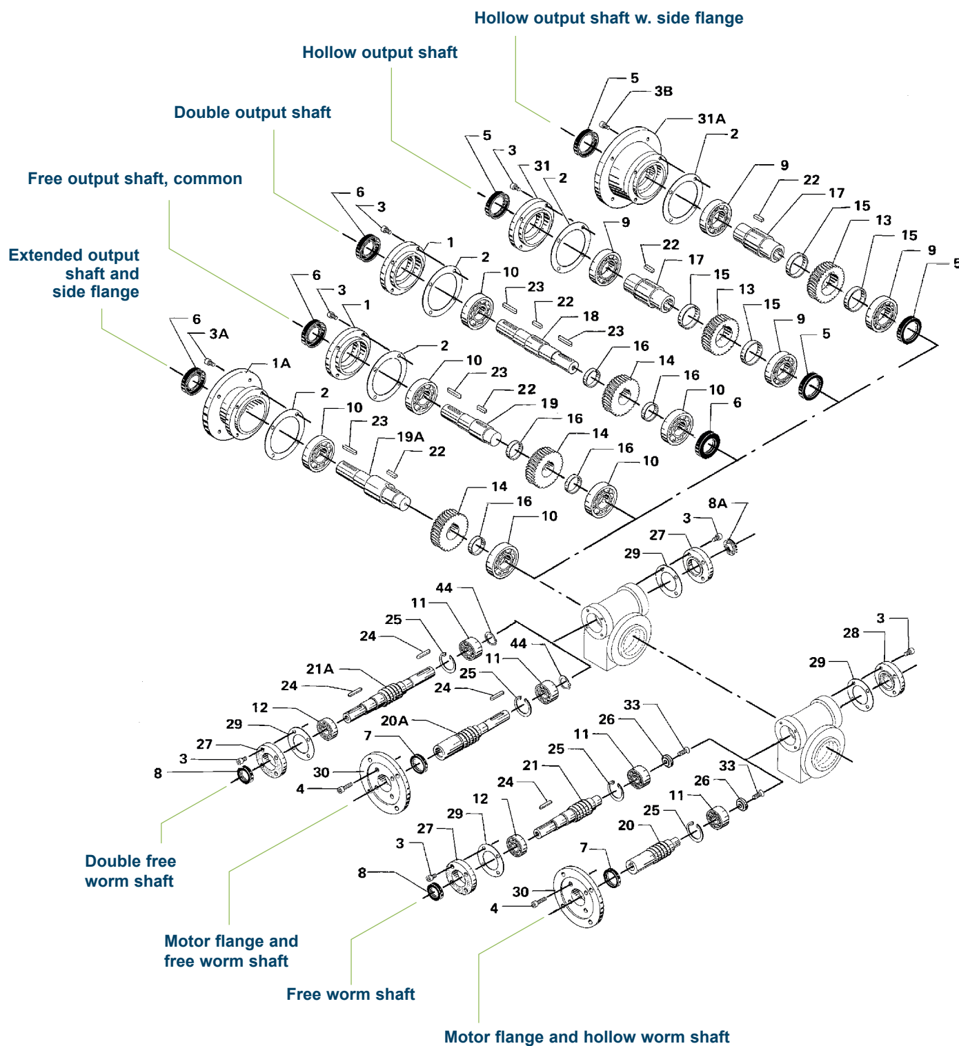
Housing type 1
